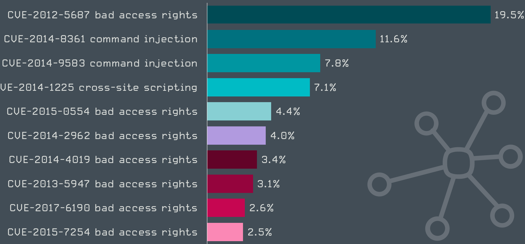
Top 10 vulnerabilities detected by ESET’s router vulnerability scanner module [% of vulnerability detections]
