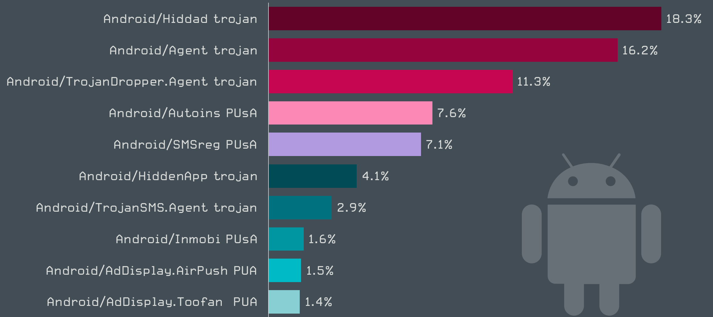
Top 10 Android threat detections in Q1 2020 [% of Android threat detections]
